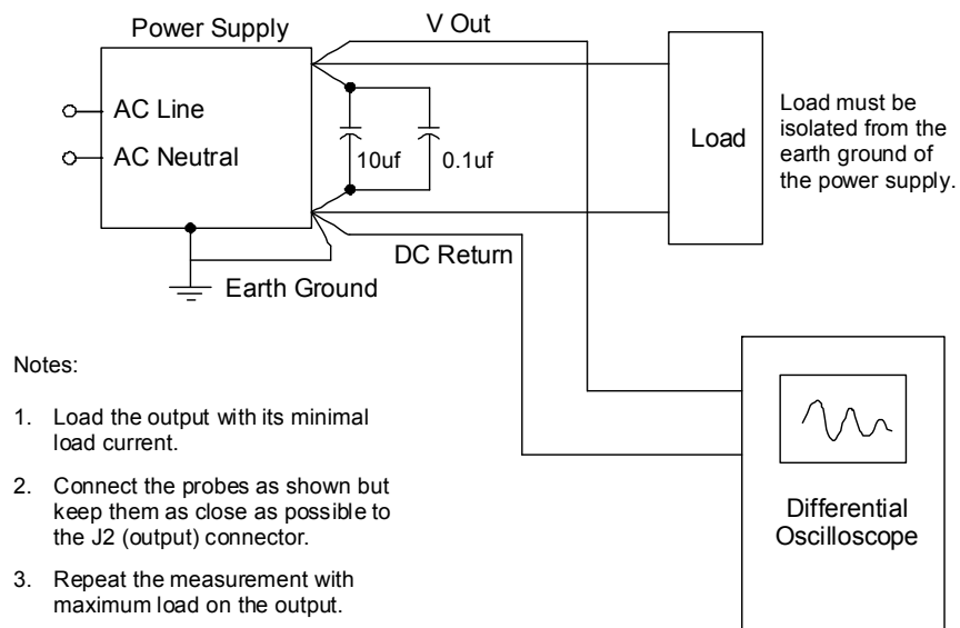
Figure 3-7 Ripple Noise Measurement Setup
