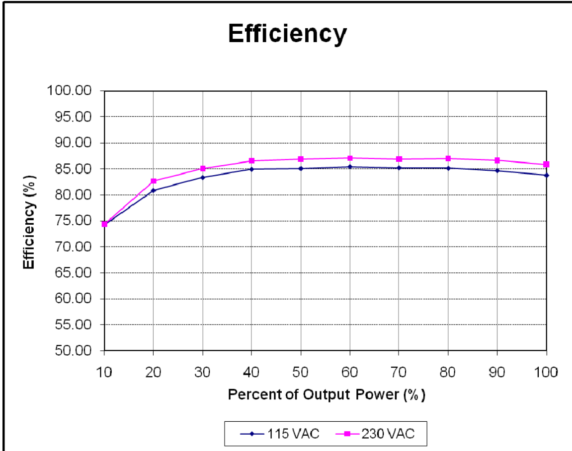
Figure 3-4 Typical Efficiency
