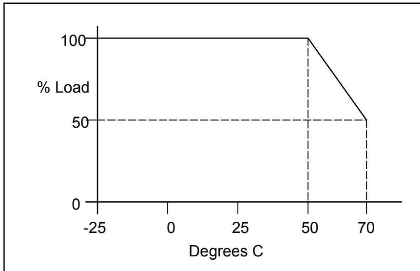
Figure 3-2 XS285ATX Output Power vs. Ambient Temperature Envelope
